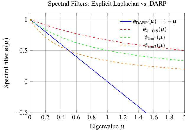
Figure 5: DARP achieves sharper low-pass filtering
